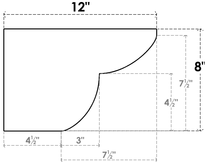
SIDE PROFILE
